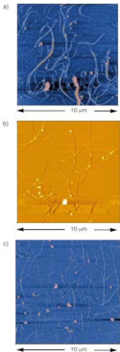
Figure 3. AFM images of bare and PmPV'-wrapped SWNTs: a) SWNTs prepared from 0.32 mg of SWNTs in 5 mL of DMF; b) solution containing 0.32 mg of SWNTs with 0.2 mg of PmPV' in 5 mL of CHCl 3 ; c) solution containing 0.24 mg of SWNTs with 1 mg of PmPV' in 5 mL of CHCl 3 .
