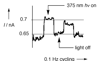
Figure 4. The performance of a PmPV'-wrapped SWNT photovoltaic device measured at 10 K. The excitation wavelength was 375 nm (slightly less than 1 mW focused to 0.2 cm 2 , with a device area of approximately 5 \times 10^{-11} cm 2 ), and a +0.025 V bias was applied to the device. Room temperature yielded a similar response if a +0.005 V bias was applied.
